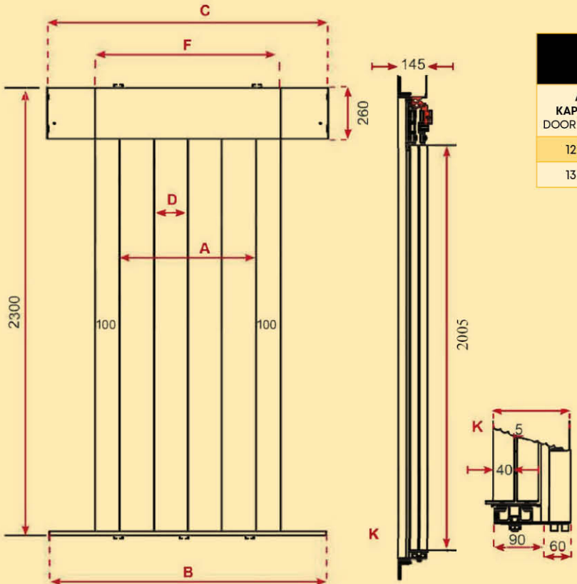
4 PANEL MERKEZİ KAT KAPISI 4 PANEL CENTRAL FLOOR DOOR
