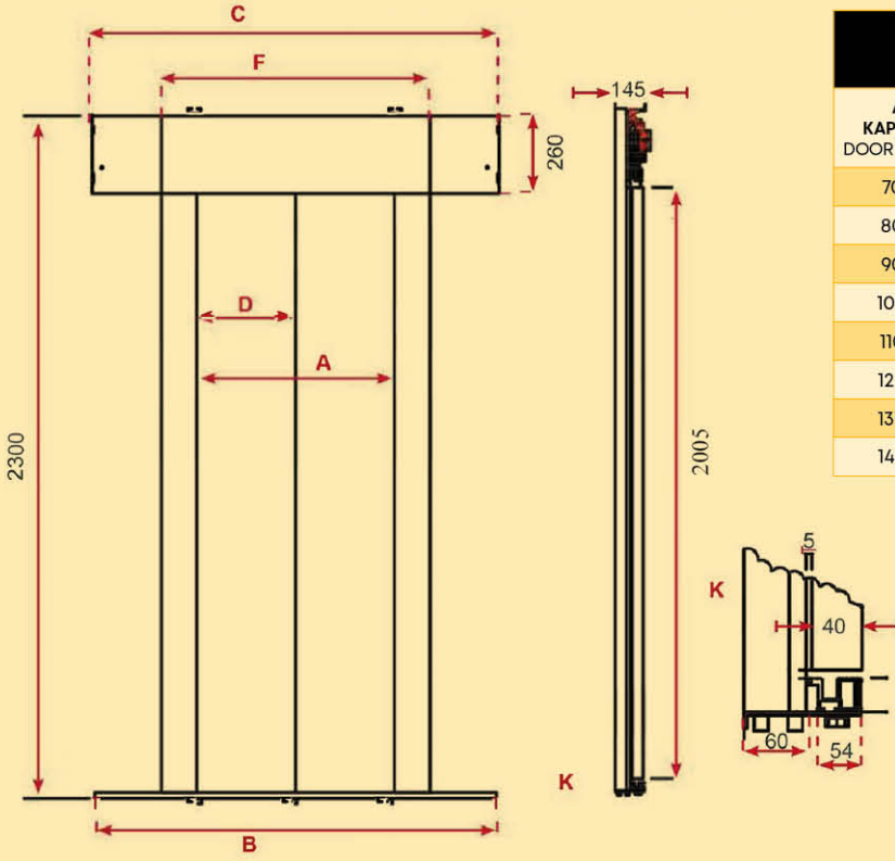
2 PANEL MERKEZİ KAT KAPISI 2 PANEL CENTRAL FLOOR DOOR
